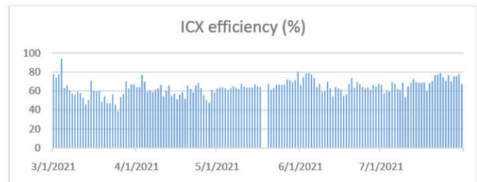
Graph 2- BIOPAQ® ICX efficiency has been registered between 55 – 70%.
