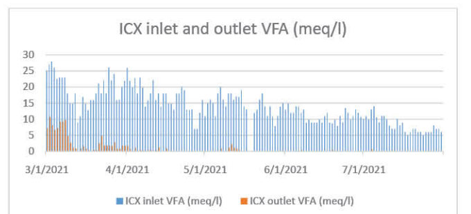
Graph 3- BIOPAQ® ICX effluent VFA is maintaining less than 5 meq/l though the influent VFA is varying from 10 to 25 meq/l. This indicates the steady state operation of BIOPAQ® ICX though there is variation of influent.
