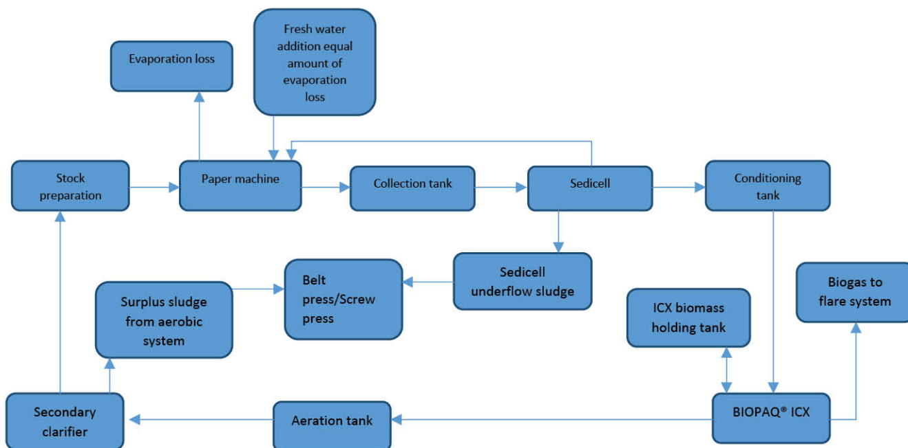
Figure 2- Closed loop circuit after BIOPAQ® ICX:
