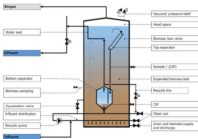
Figure 1- Schematic overview of BIOPAQ® ICX reactor
